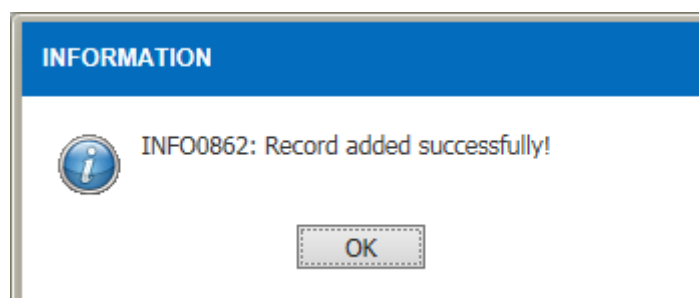
Figure 3.1.3-3 Confirmation Alert
