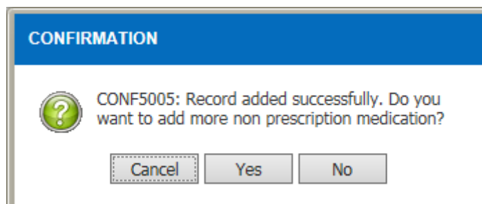
Figure 3.1.2-8 Confirmation Alert
