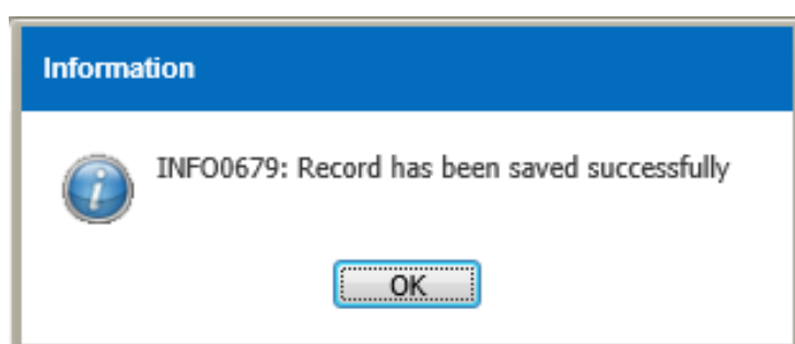
Figure 3.11.2-7 Information Message
