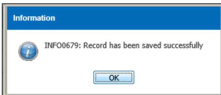
Figure 3.9.1-4 Information Message
