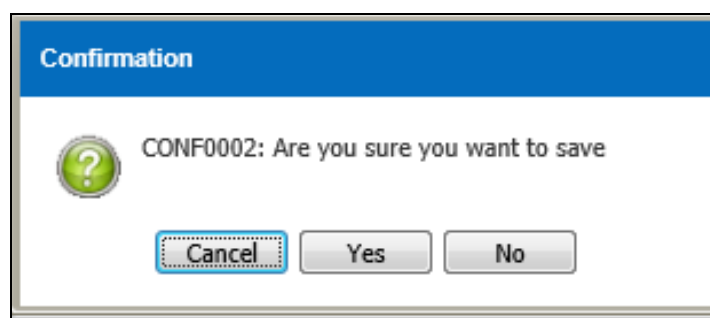
Figure 3.5.2-4 Confirmation Message
