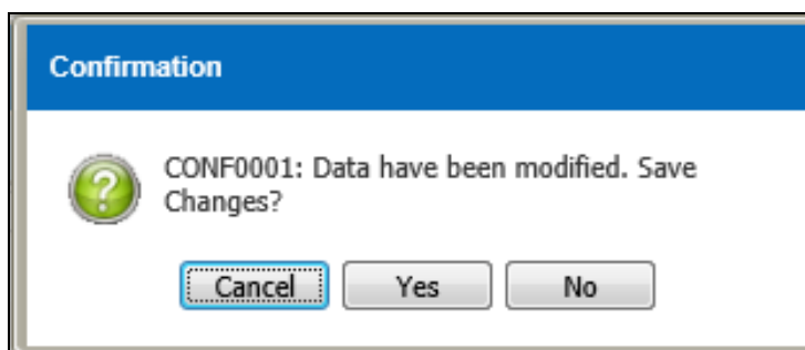
Figure 3.11.2-6 Confirmation Message
