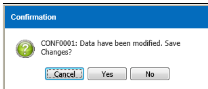
Figure 3.10.2-4 Confirmation Message
