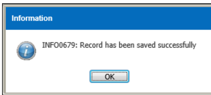
Figure 3.13.1-4 Information Message
