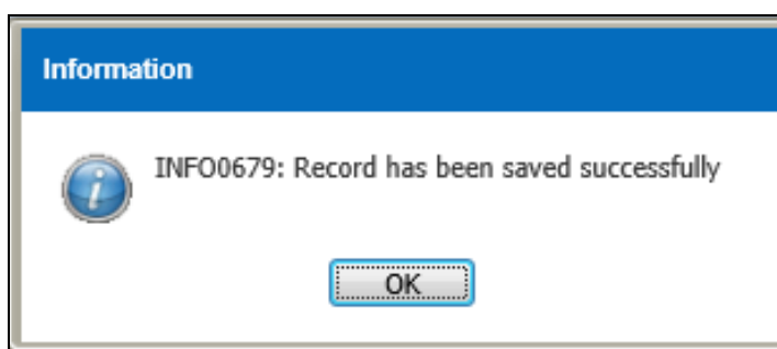
Figure 3.5.1-4 Information Message
