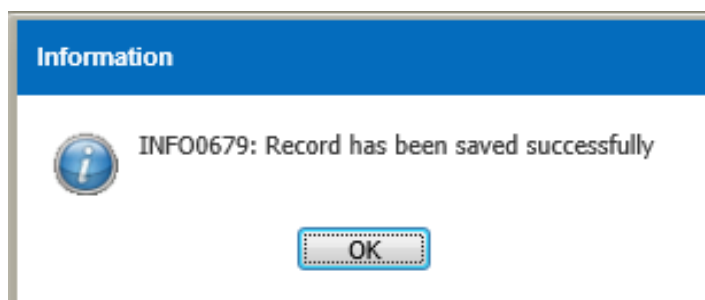
Figure 3.6.1-4 Information Message
