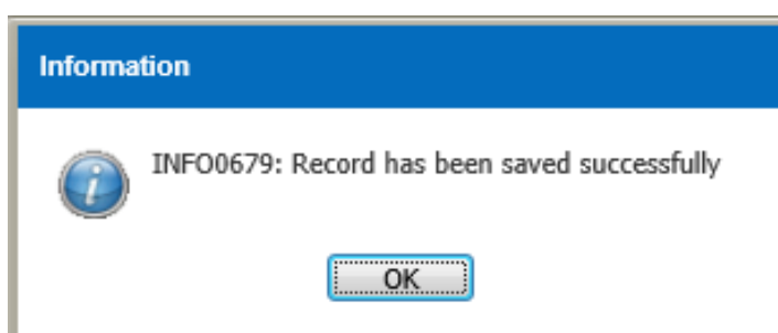
Figure 3.12.1-4 Information Message
