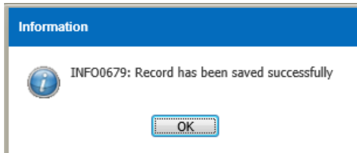
Figure 3.11.1-5 Information Message
