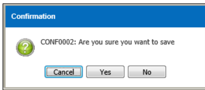
Figure 3.7.1-3 Confirmation Message
