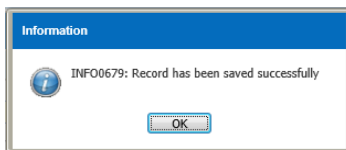
Figure 3.2.2-4 Information Message
