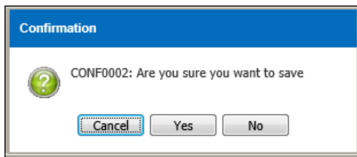
Figure 3.10.1-3 Confirmation Message
