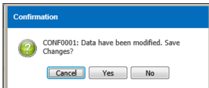
Figure 3.8.2-4 Confirmation Message
