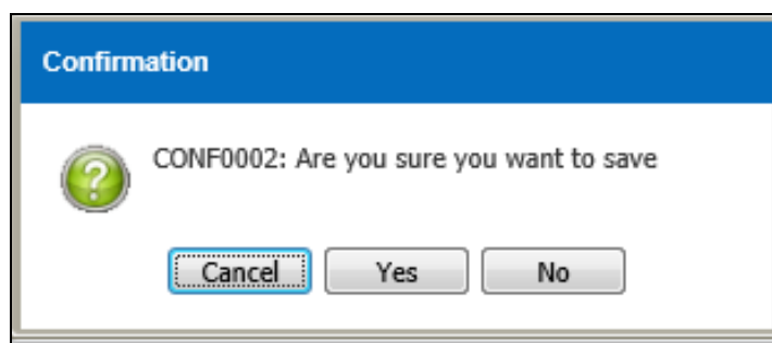
Figure 3.8.1-3 Confirmation Message
