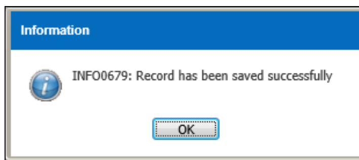
Figure 3.4.2-5 Information Message
