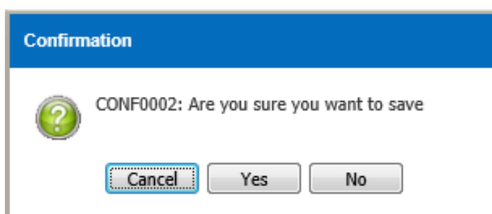
Figure 3.12.1-3 Confirmation Message
