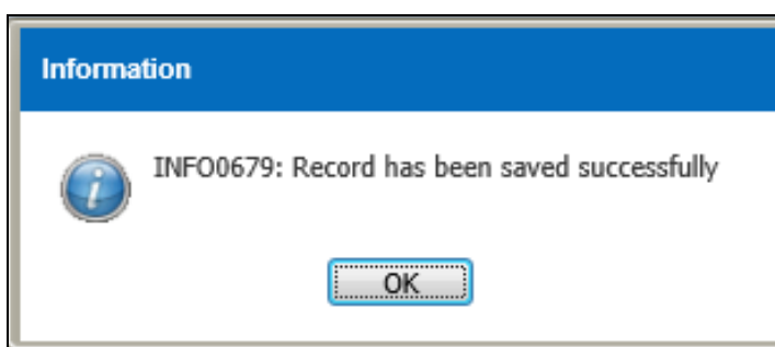
Figure 3.2.1-4 Information Message
