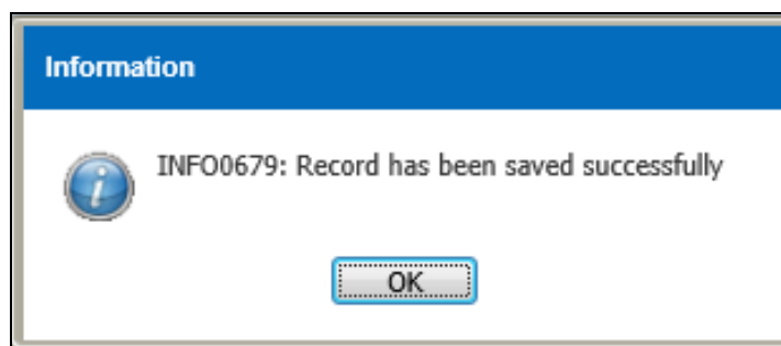
Figure 3.10.1-4 Information Message
