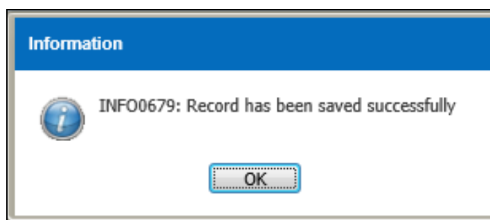
Figure 3.13.2-5 Information Message
