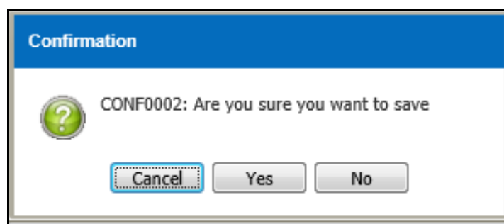
Figure 3.6.1-3 Confirmation Message
