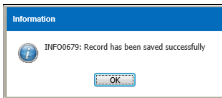
Figure 3.7.1-4 Information Message
