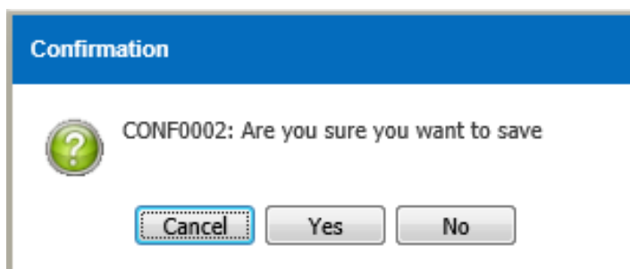
Figure 3.11.1-4 Confirmation Message
