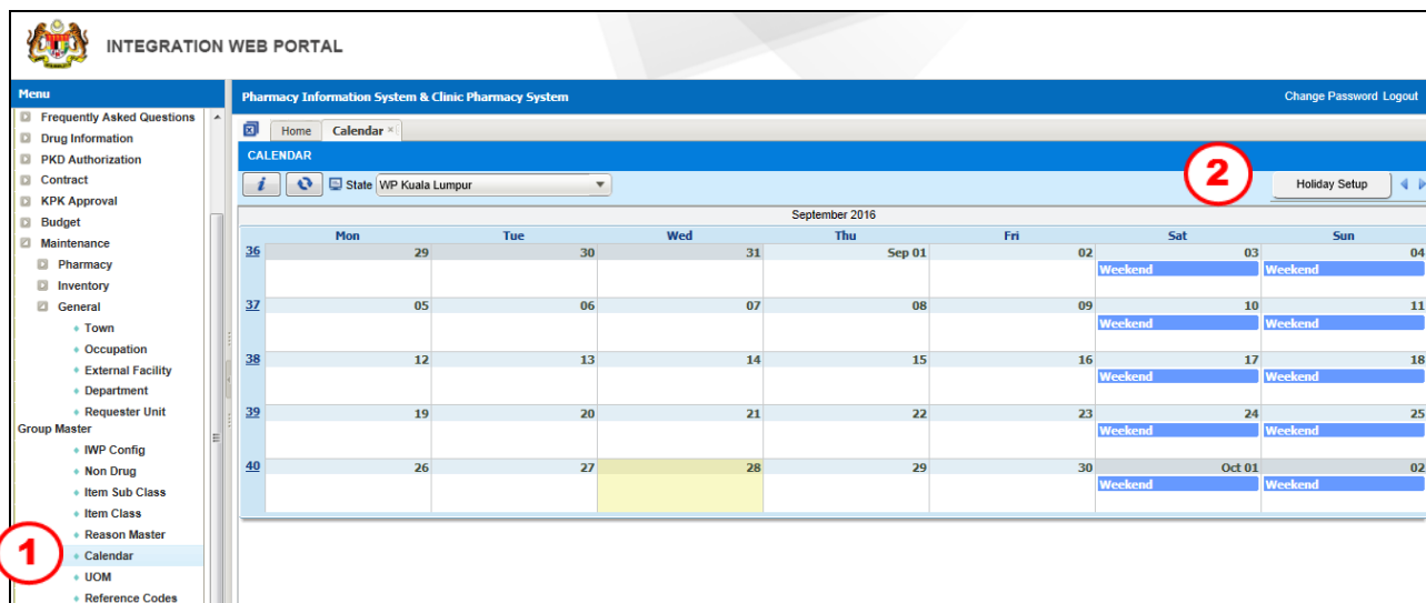
Figure 3.11.2-1 Calendar
