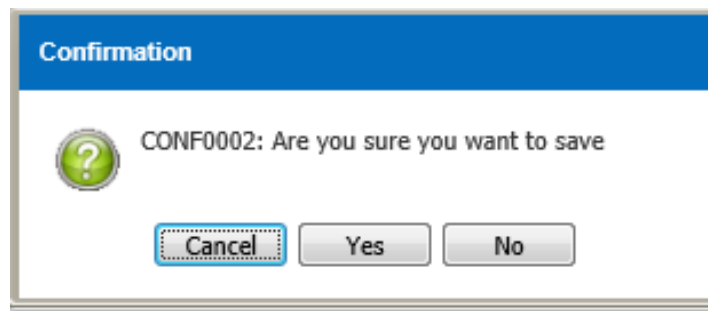
Figure 3.13.2-4 Confirmation Message
