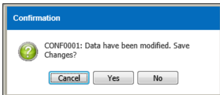
Figure 3.7.2-4 Confirmation Message
