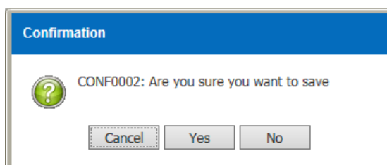
Figure 3.18.1-5 Confirmation Message
