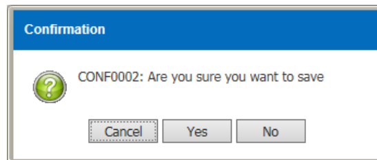
Figure 3.17.1-5 Confirmation Message
