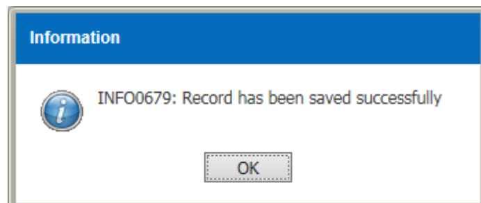
Figure 3.5.1-4 Information Message
