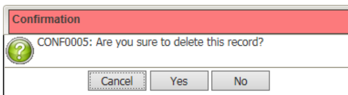
Figure 3.18.2-6 Confirmation Message
