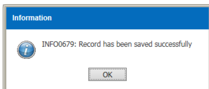
Figure 3.10.1-5 Information Message
