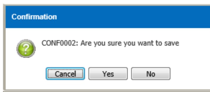
Figure 3.9.1-14 Confirmation Message
