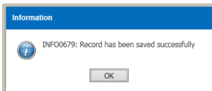
Figure 3.3.2-4 Information Message
