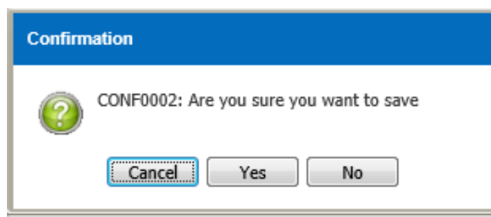
Figure 3.2.1-5 Confirmation Message
