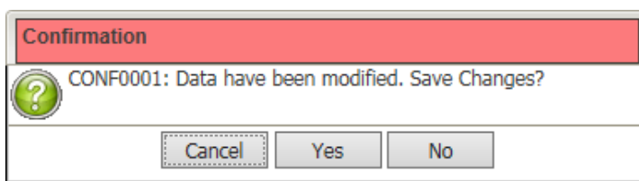
Figure 3.18.2-4 Confirmation Message
