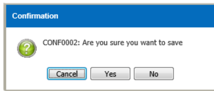
Figure 3.6.1-4 Confirmation Message
