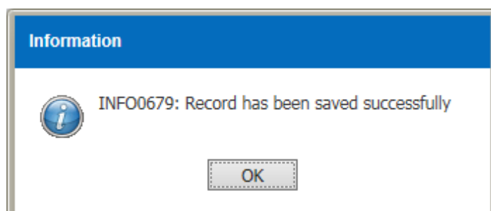
Figure 3.4.1-6 Information Message
