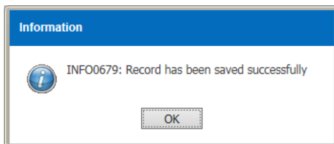
Figure 3.6.2-4 Information Message
