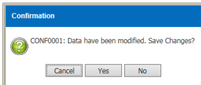
Figure 3.10.2-4 Confirmation Message
