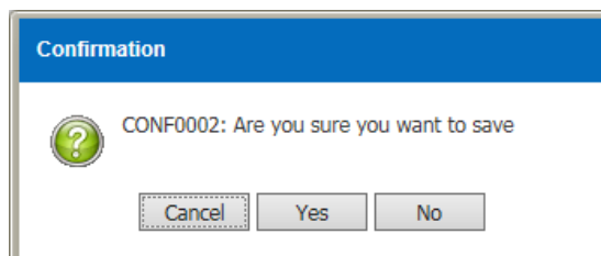
Figure 3.16.1-8 Confirmation Message
