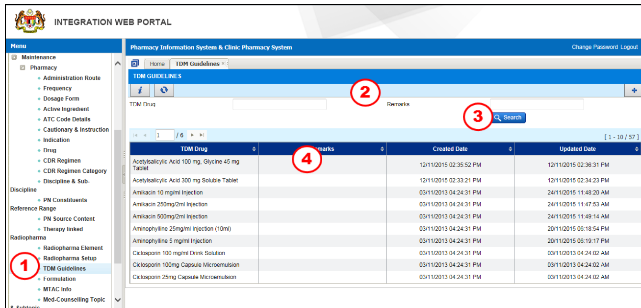
Figure 3.16.2-1 TDM Guideline
