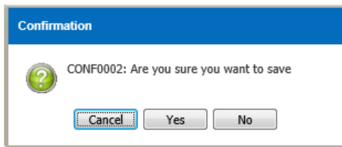
Figure 3.11.1-7 Confirmation Message
