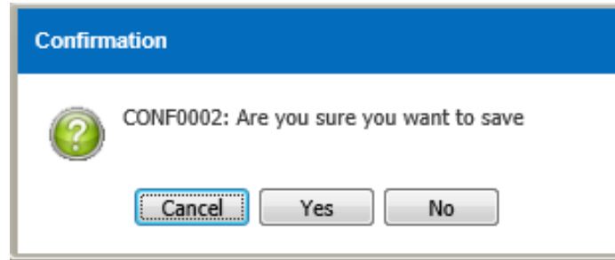
Figure 3.5.1-3 Confirmation Message
