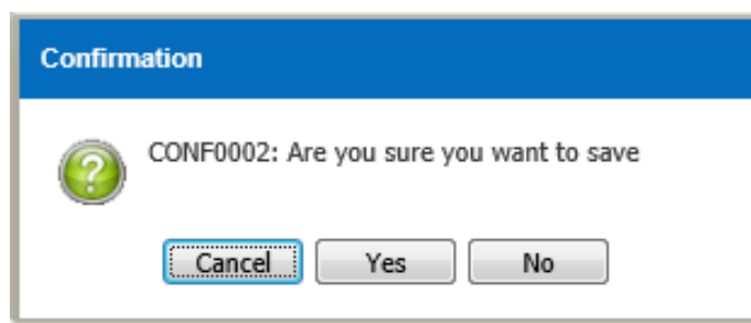
Figure 3.10.1-4 Confirmation Message
