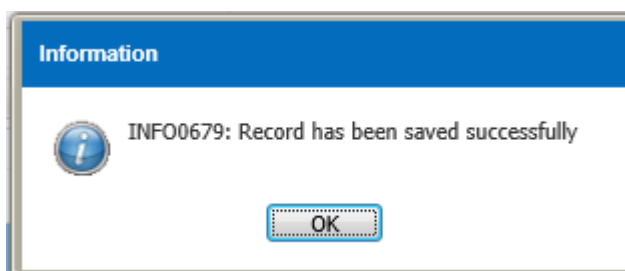
Figure 3.9.1-5 Confirmation Message
