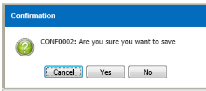
Figure 3.9.2-4 Confirmation Message
