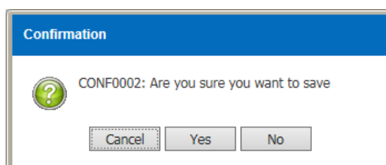
Figure 3.16.1-10 Confirmation Message
