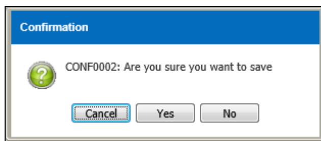
Figure 3.9.1-12 Confirmation Message
