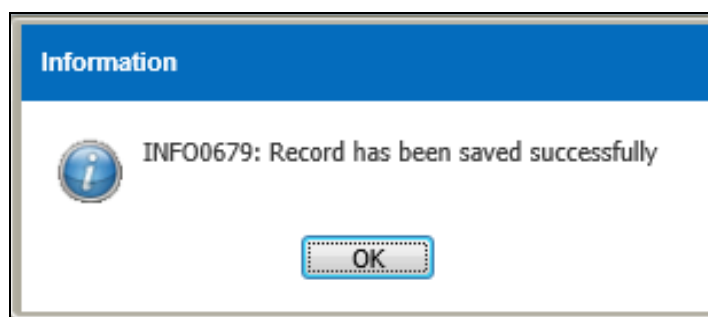
Figure 3.9.1-15 Information Message
