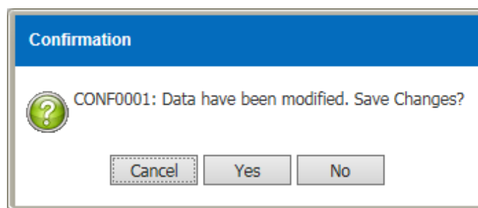
Figure 3.16.2-4 Confirmation Message
