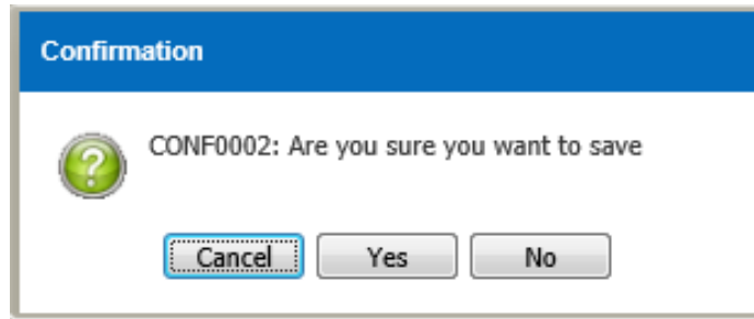
Figure 3.3.1-3 Confirmation Message
