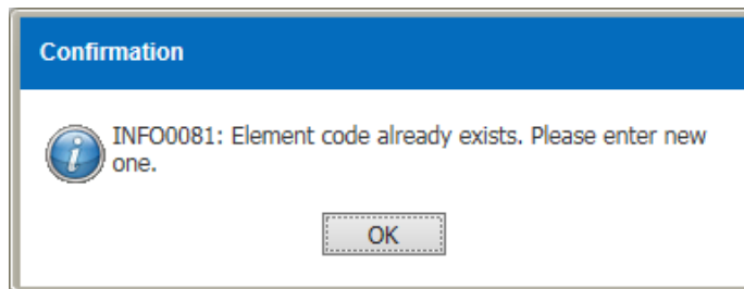
Figure 3.15.1-8 Information Message
