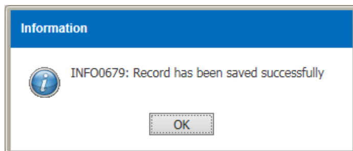
Figure 3.3.1-4 Information Message
