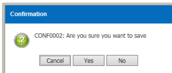
Figure 3.18.1-9 Confirmation Message
