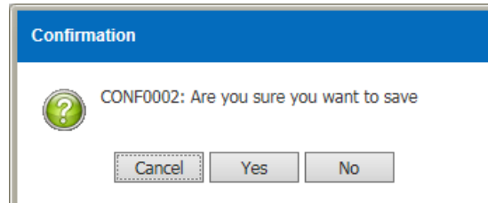
Figure 3.14.1-5 Confirmation Message
