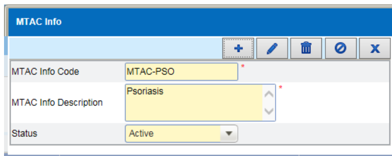
Figure 3.17.1-2 MTAC Info
