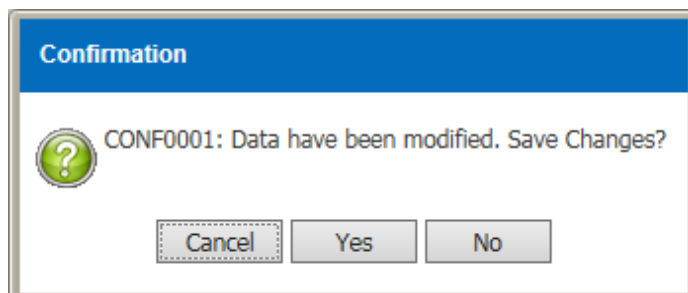
Figure 3.12-9 Confirmation Message
