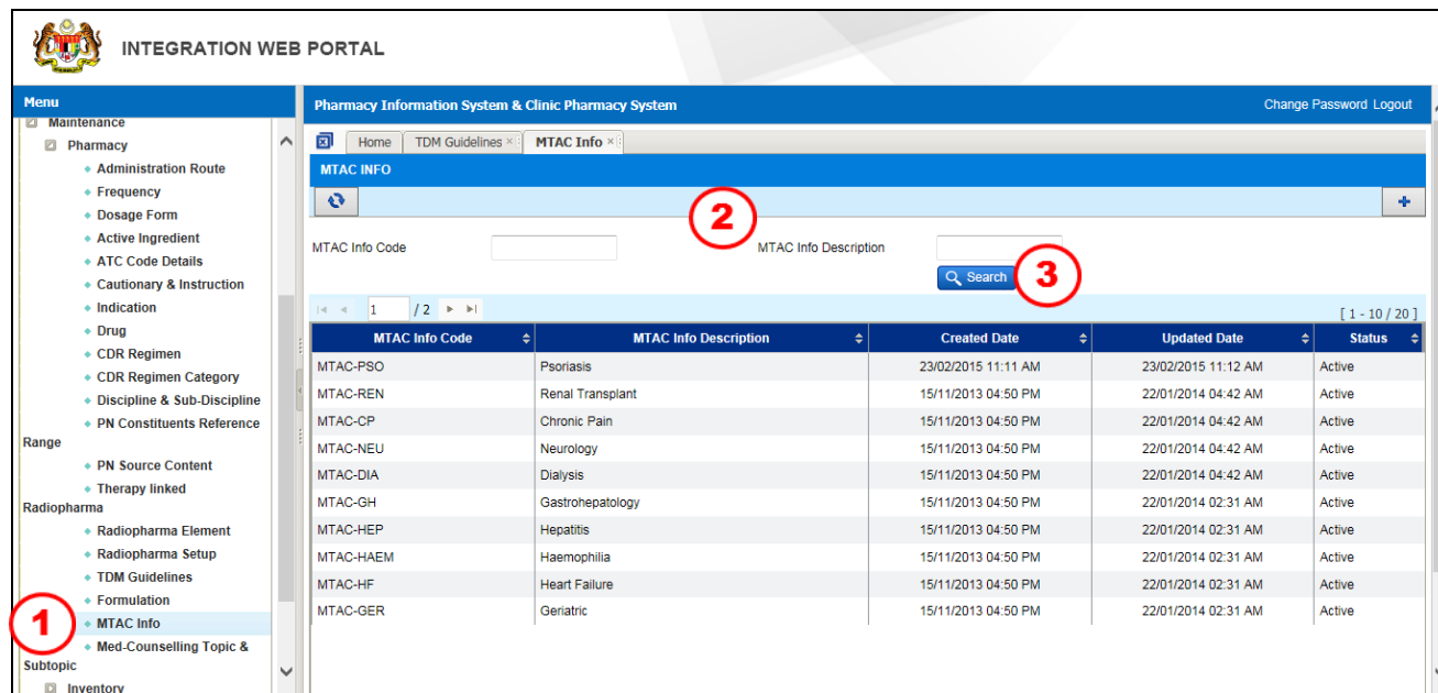
Figure 3.17.1-1 MTAC Info
