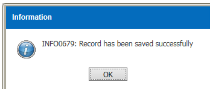
Figure 3.12-10 Information Message
