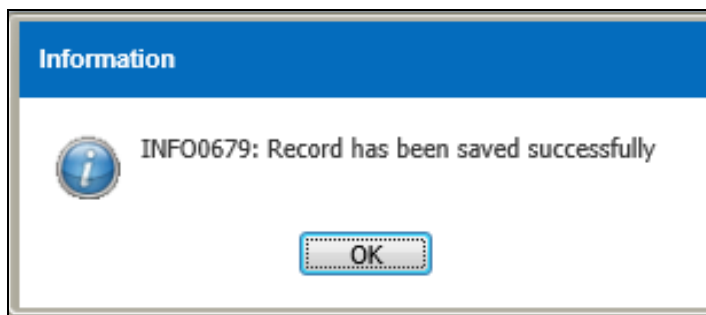
Figure 3.9.2-5 Confirmation Message
