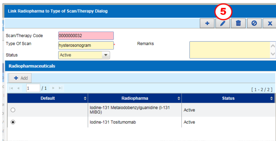
Figure 3.14.2-2 Link Radiopharma to Type of Scan/Therapy Dialog
